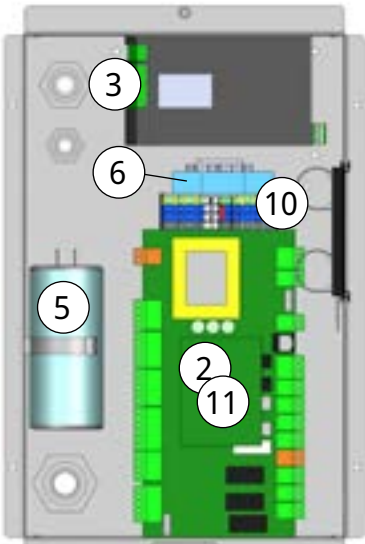
EcoHeat 406-412 1x230V
